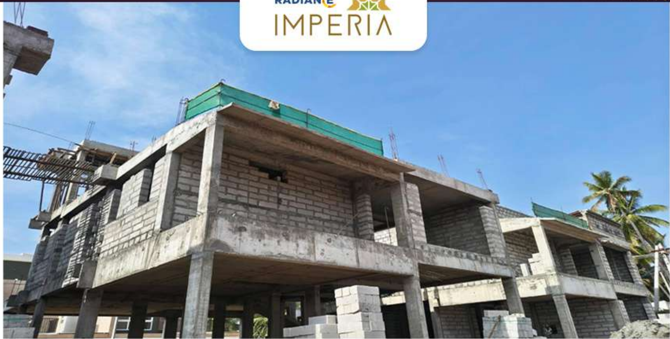
Villa 16 Block Work in Progress
