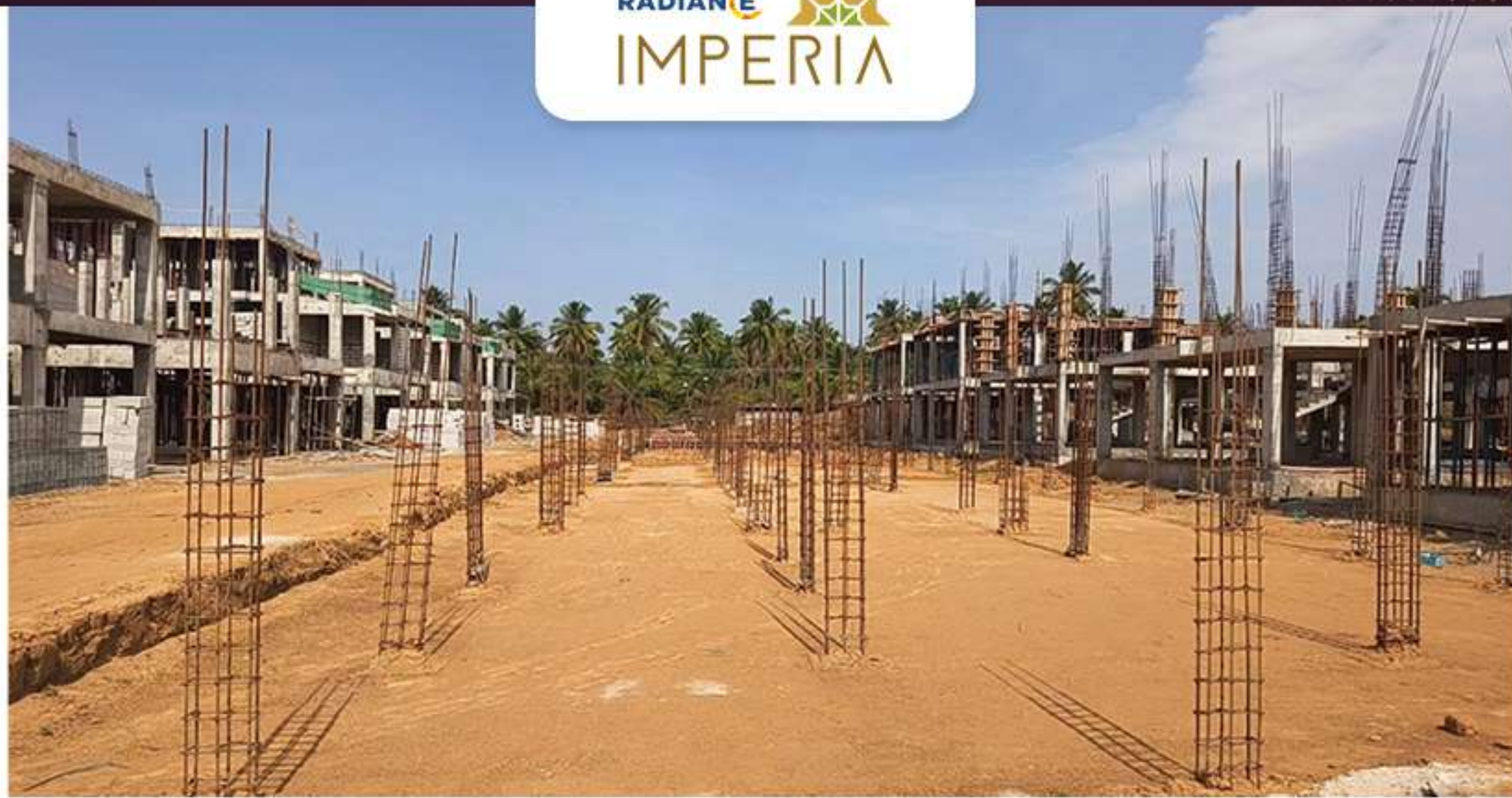
Villas 79-75: Soil compaction work in progress
