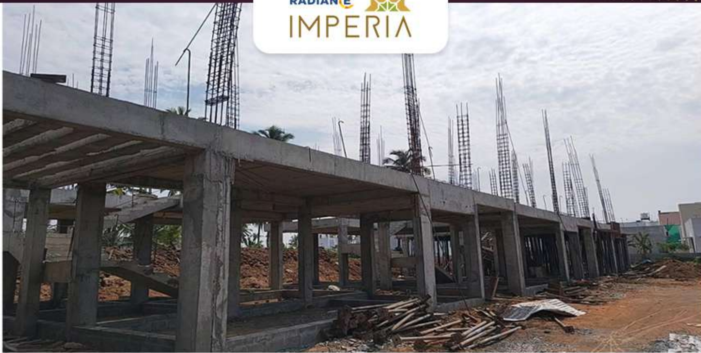
Villas- 95 1st Floor Column Work in Progress
