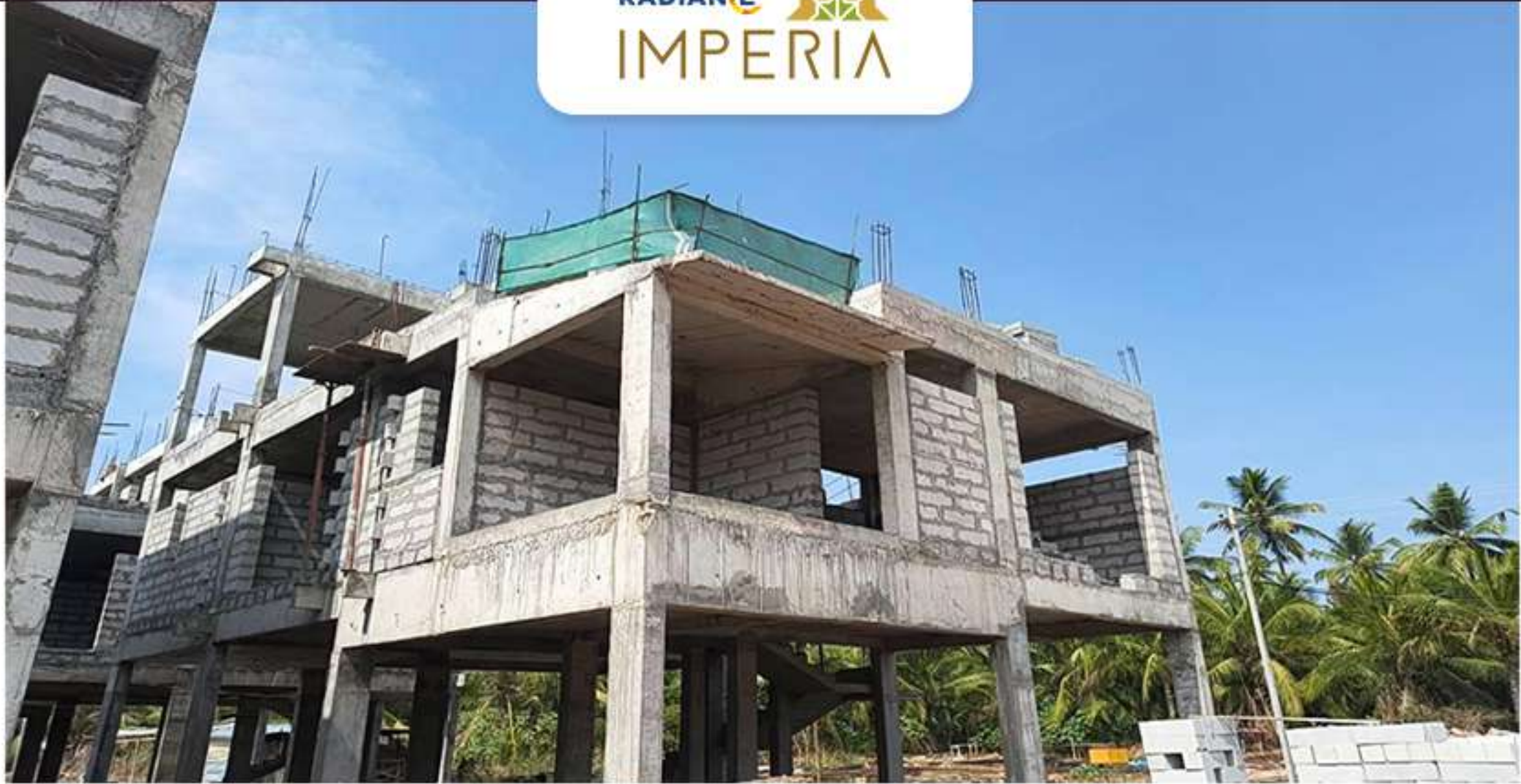
Villas-72 Block Work in Progress
