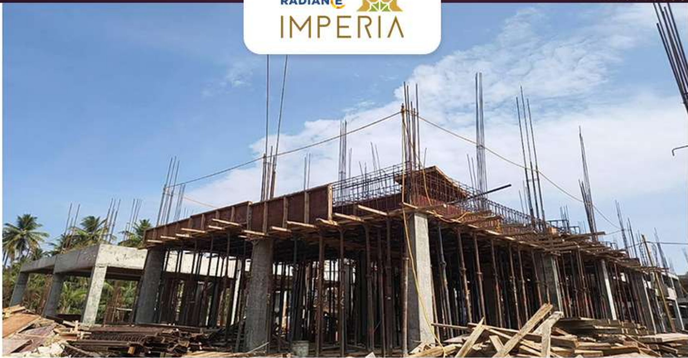
Villa 22 Ground Floor Roof Slab Work in Progress
