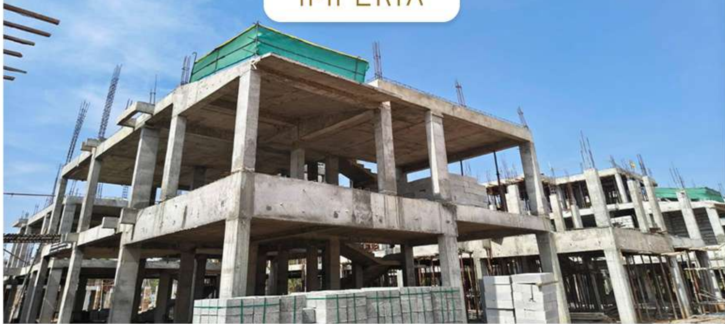
Villas-66 2nd Floor Column Work in Progress
