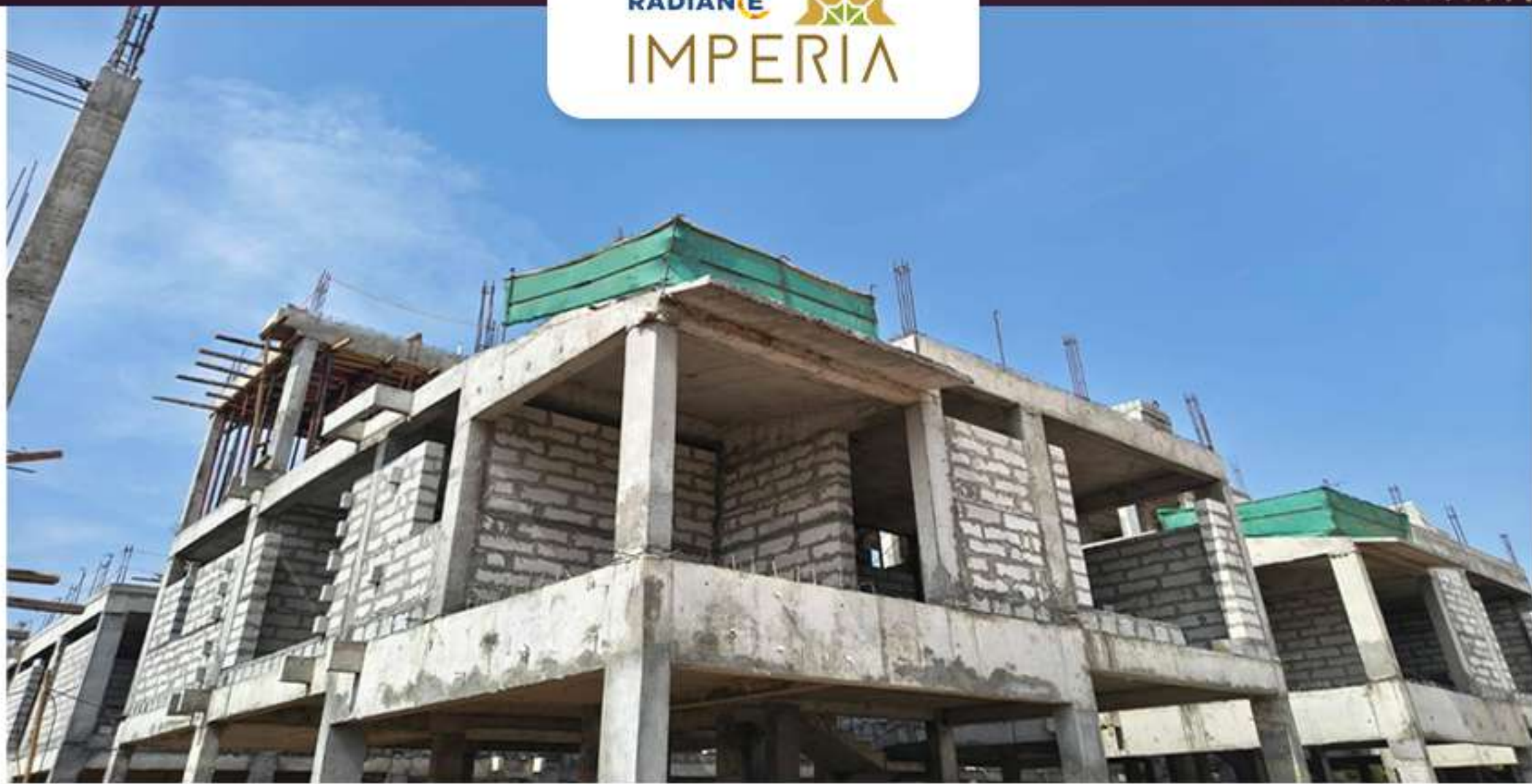
Villas-69 Block Work in Progress
