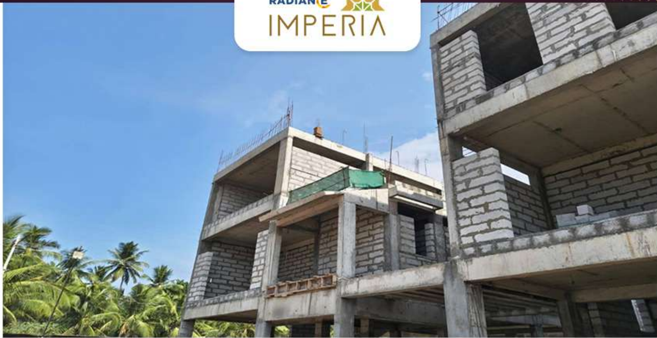
Villa 45 Block Work in Progress
