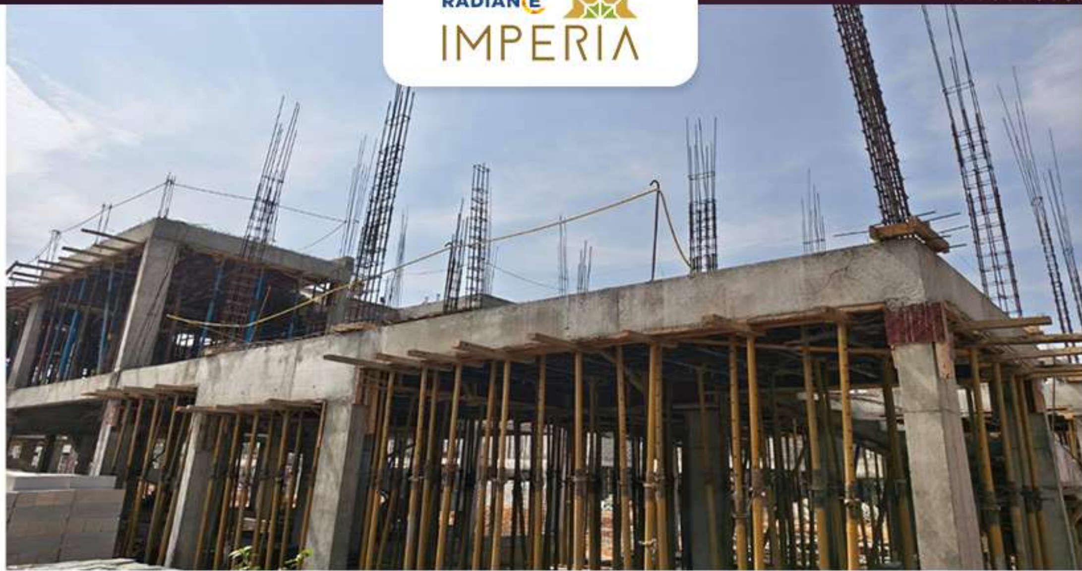
Villas-87 1st Floor Column Work in Progress
