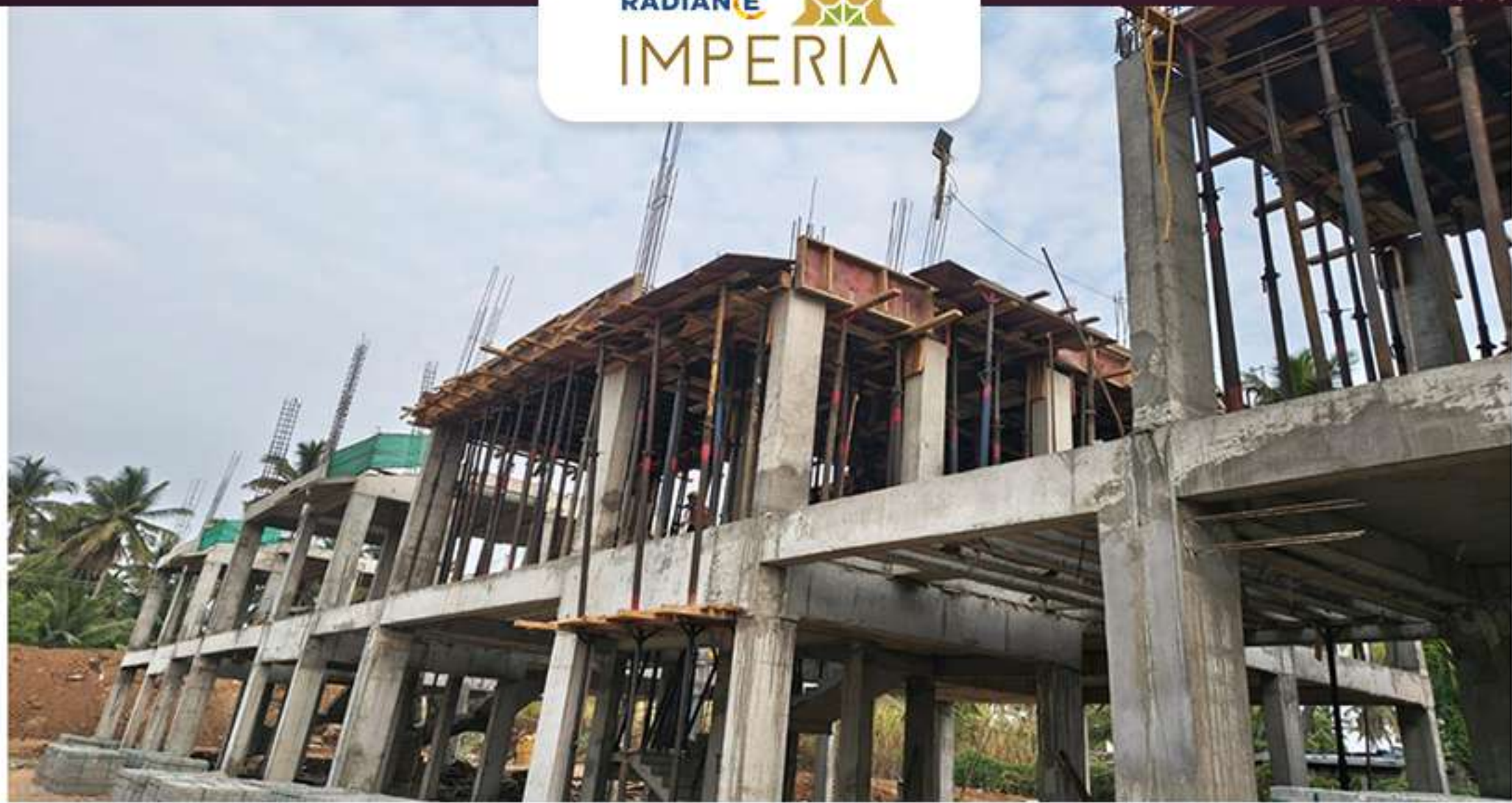
Villa 91 1st Floor Roof Slab Shuttering Work in Progress
