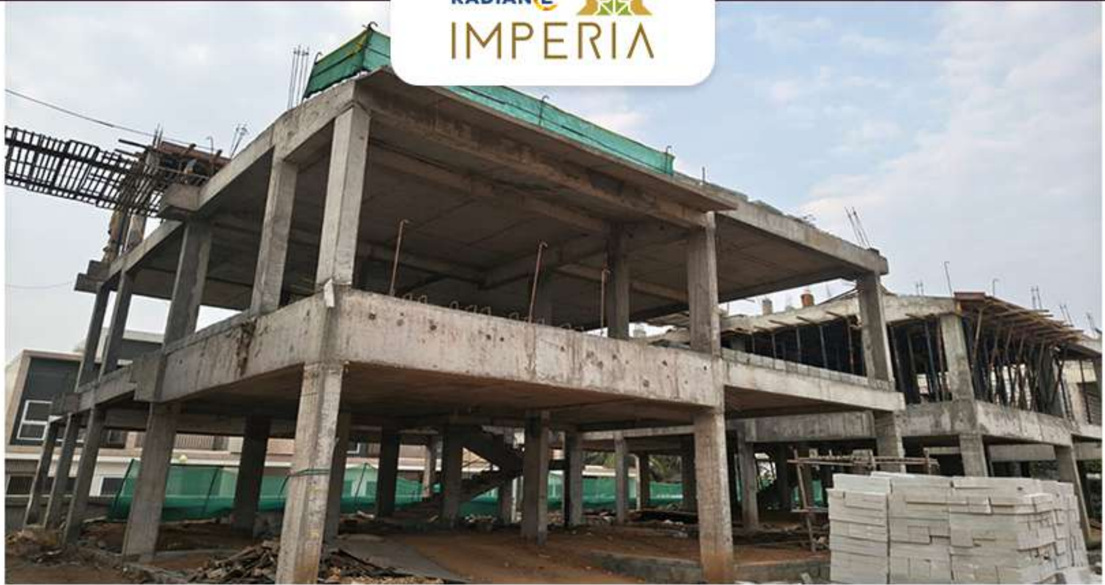
Villa no. 15 2nd Floor roof Slab Shuttering Work in Progress
