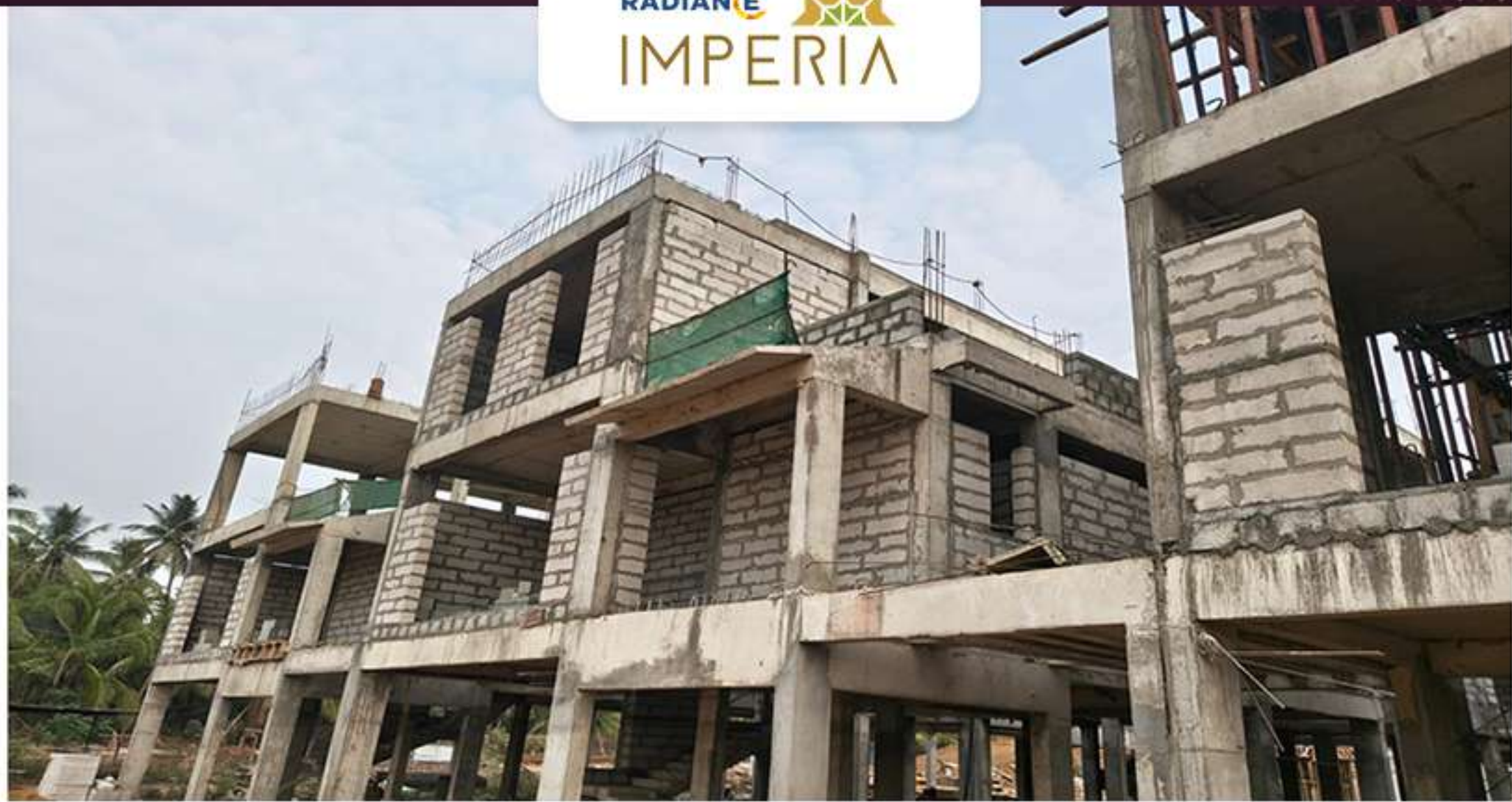
Villa 46 Block Work in Progress
