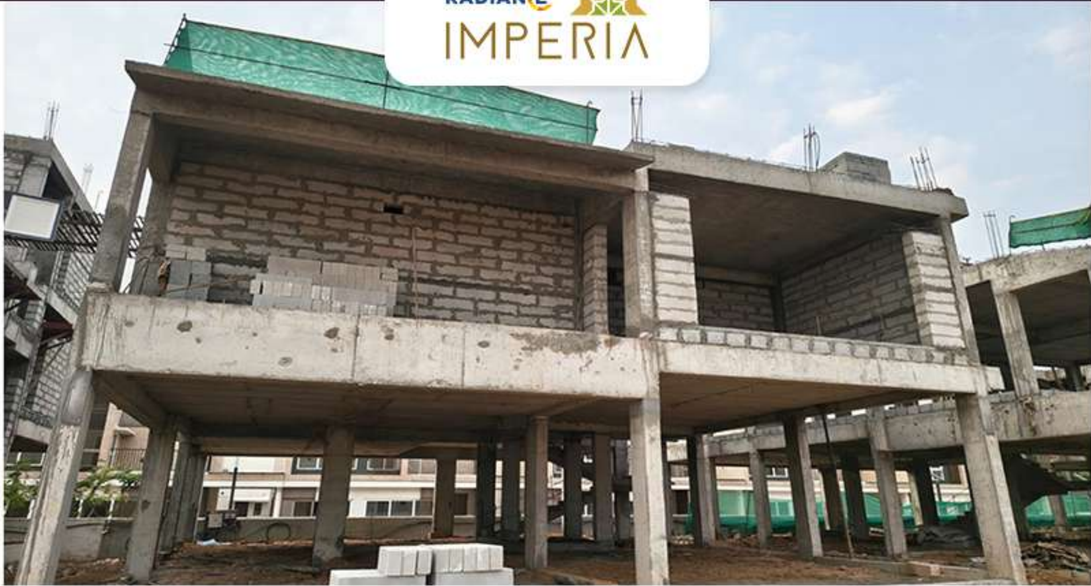
Villa no 14 Block Work is Work in Progress
