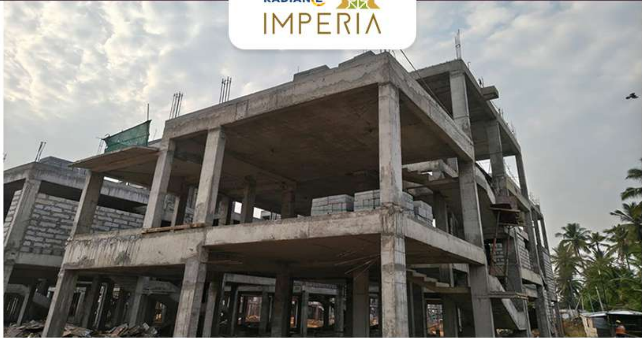
Villa 72 Block Work in Progress
