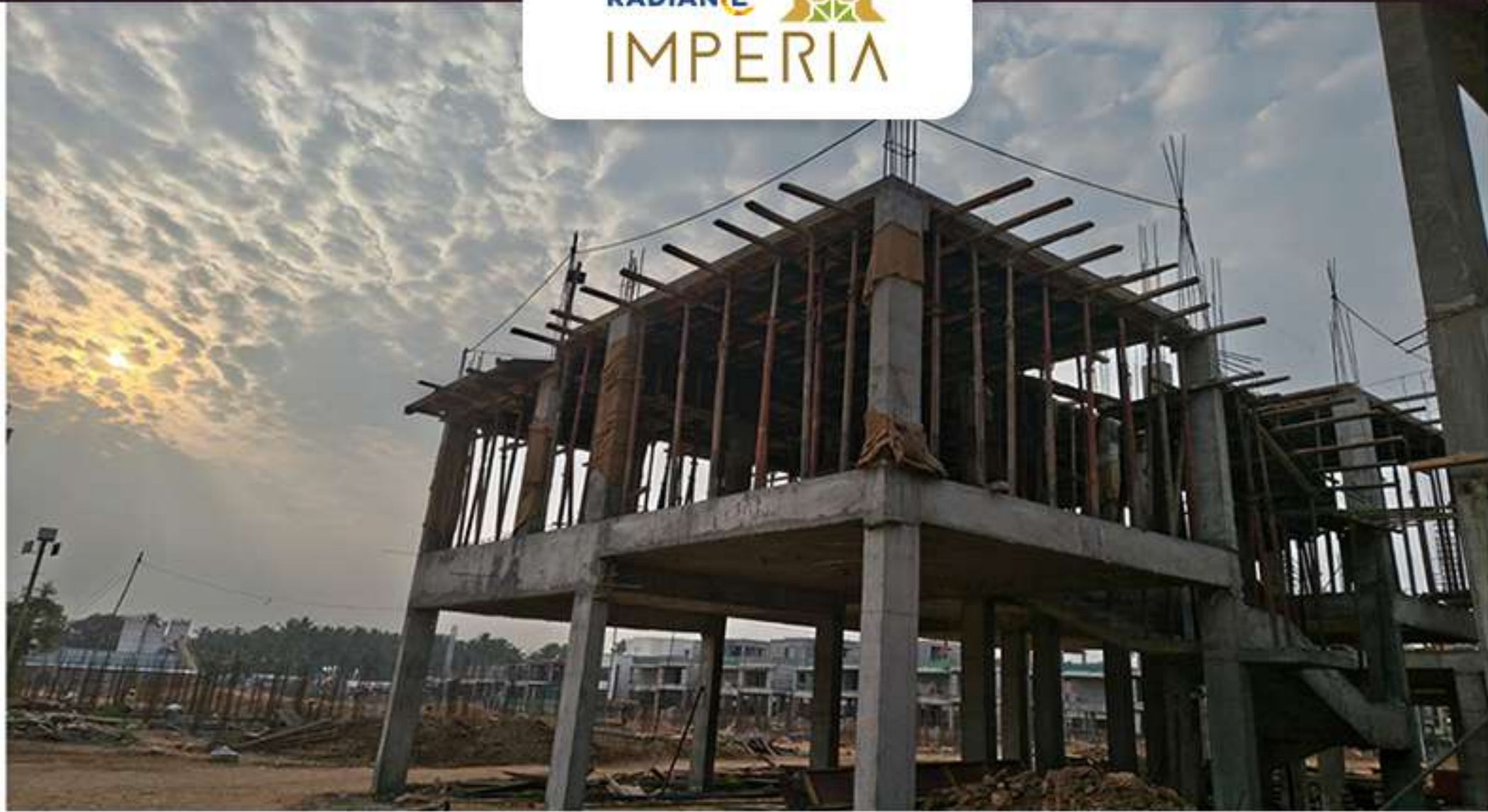
Villa 65 1st Floor Roof Slab Work in Progress
