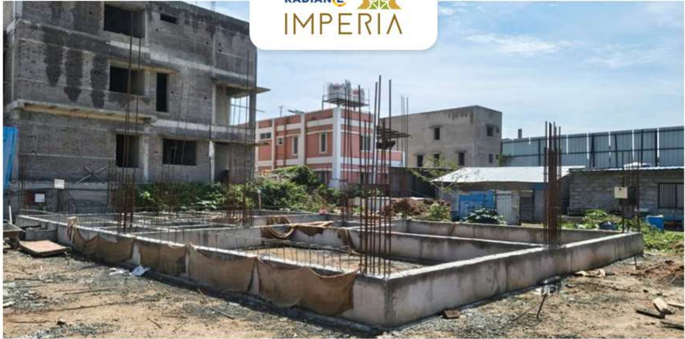
Villa no 64 Plinth Beam Completed
