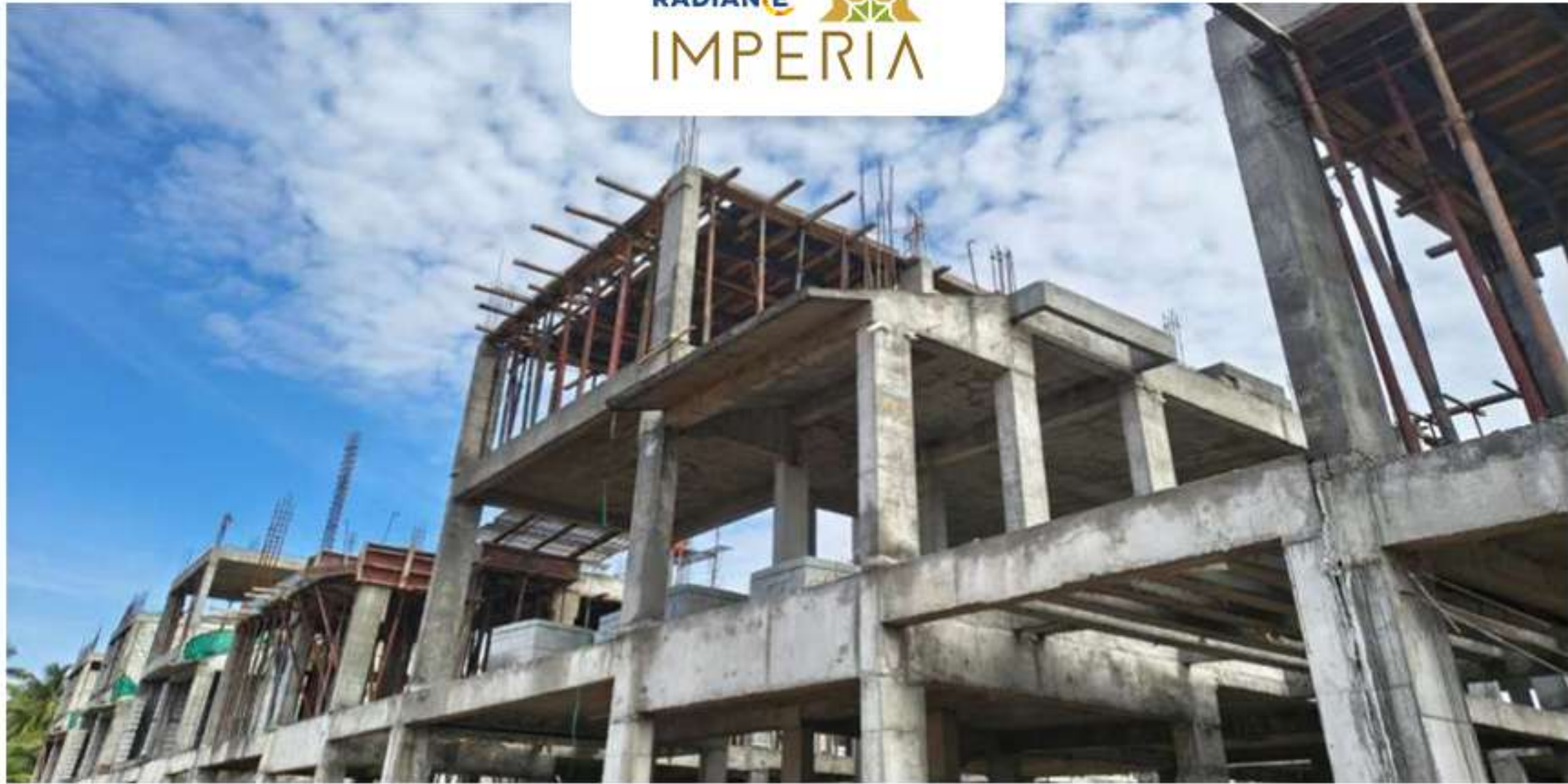
Villa no -50 2nd Floor Roof Slab Shuttering work in Progress
