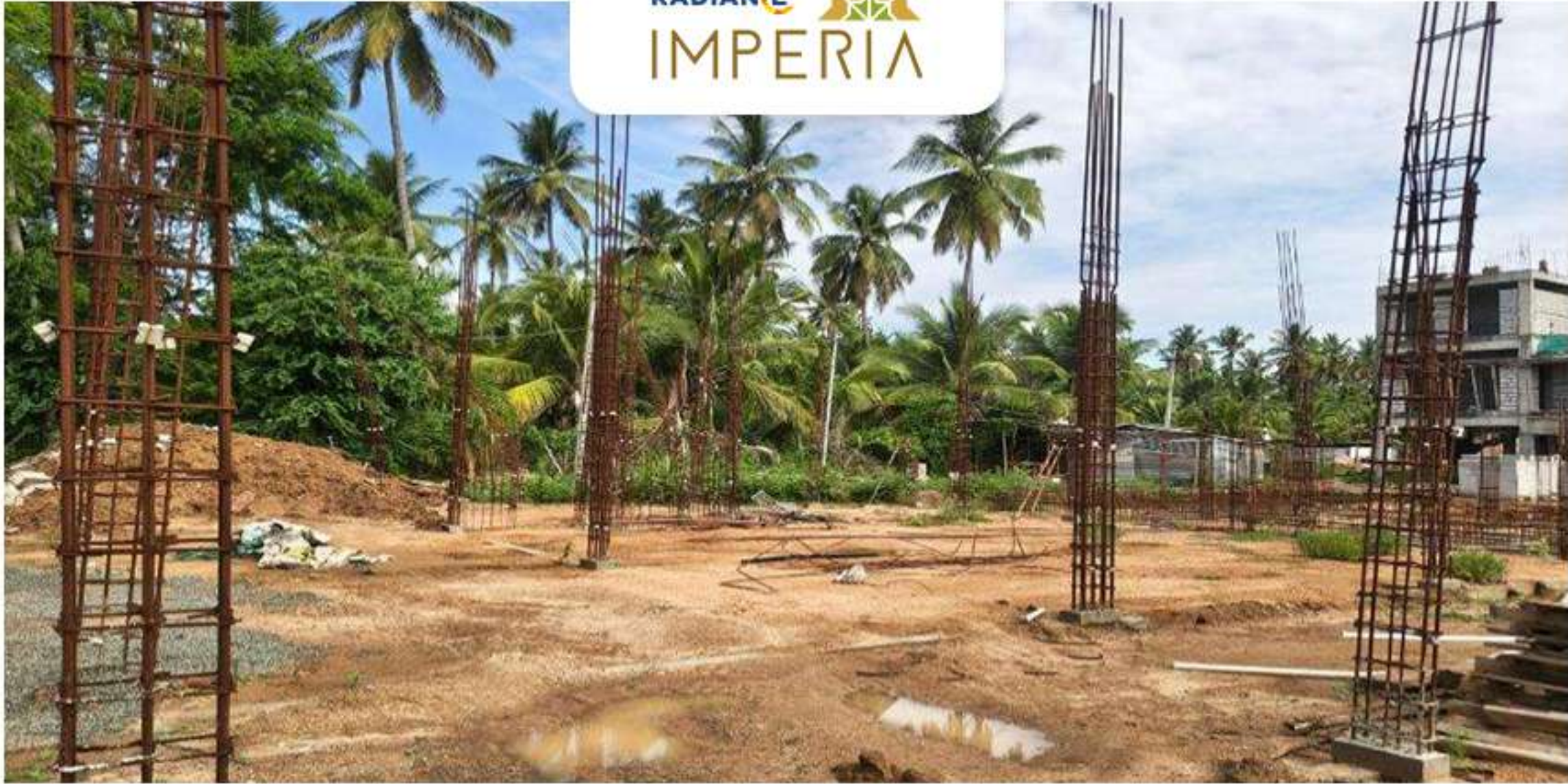
Villa no -19 Ground Floor Column Reinforcement Work in Progress
