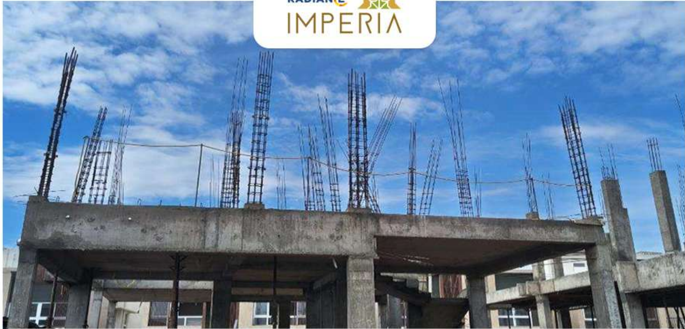
Villa no. 1 -1st Floor Column Work in Progress
