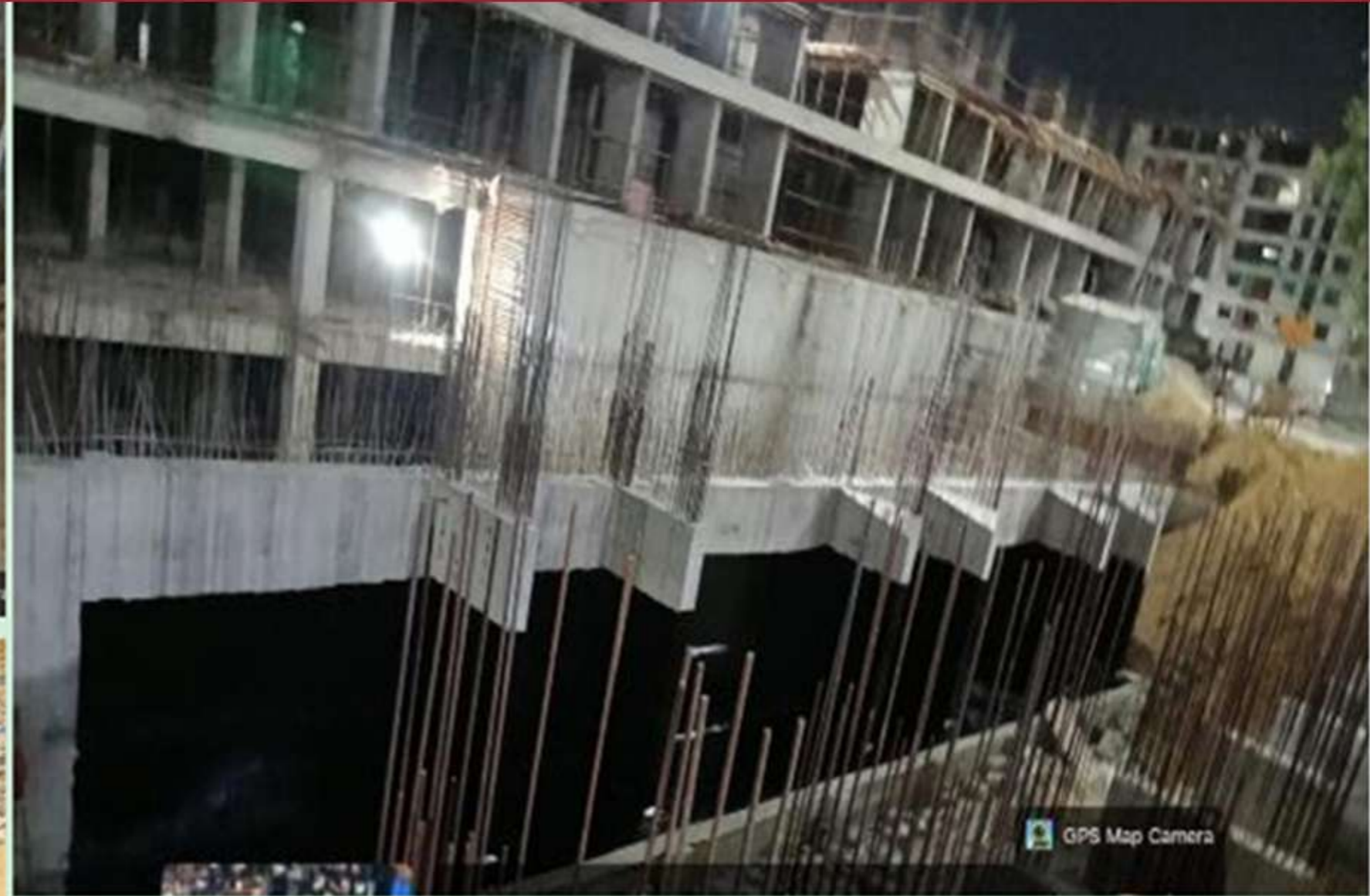
STP - West side retaining wall area, Primer & SBS Membrane laying
