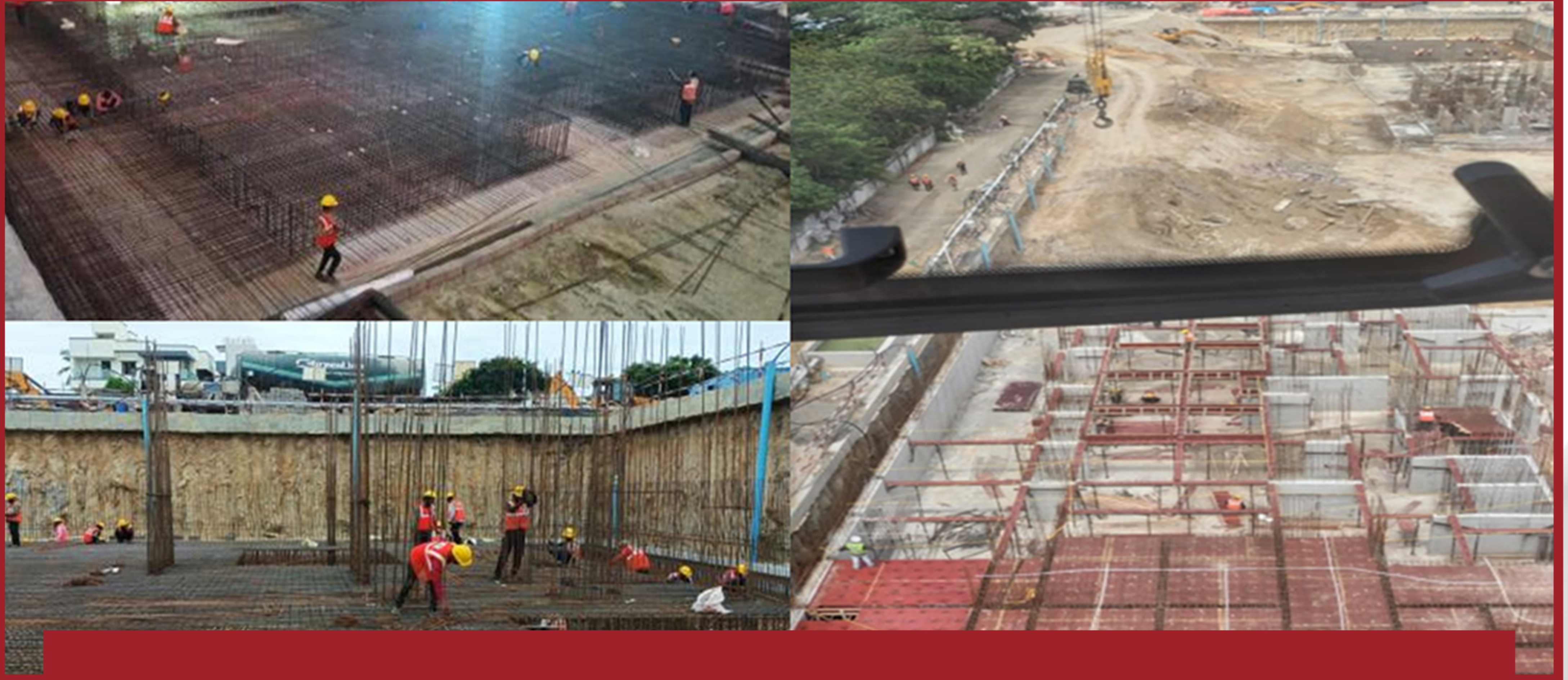
Block B – Raft Part 2 Reinforcement Works ( Concrete Plan 29.9.25 / 640cum ) And Part 3 Excavation
