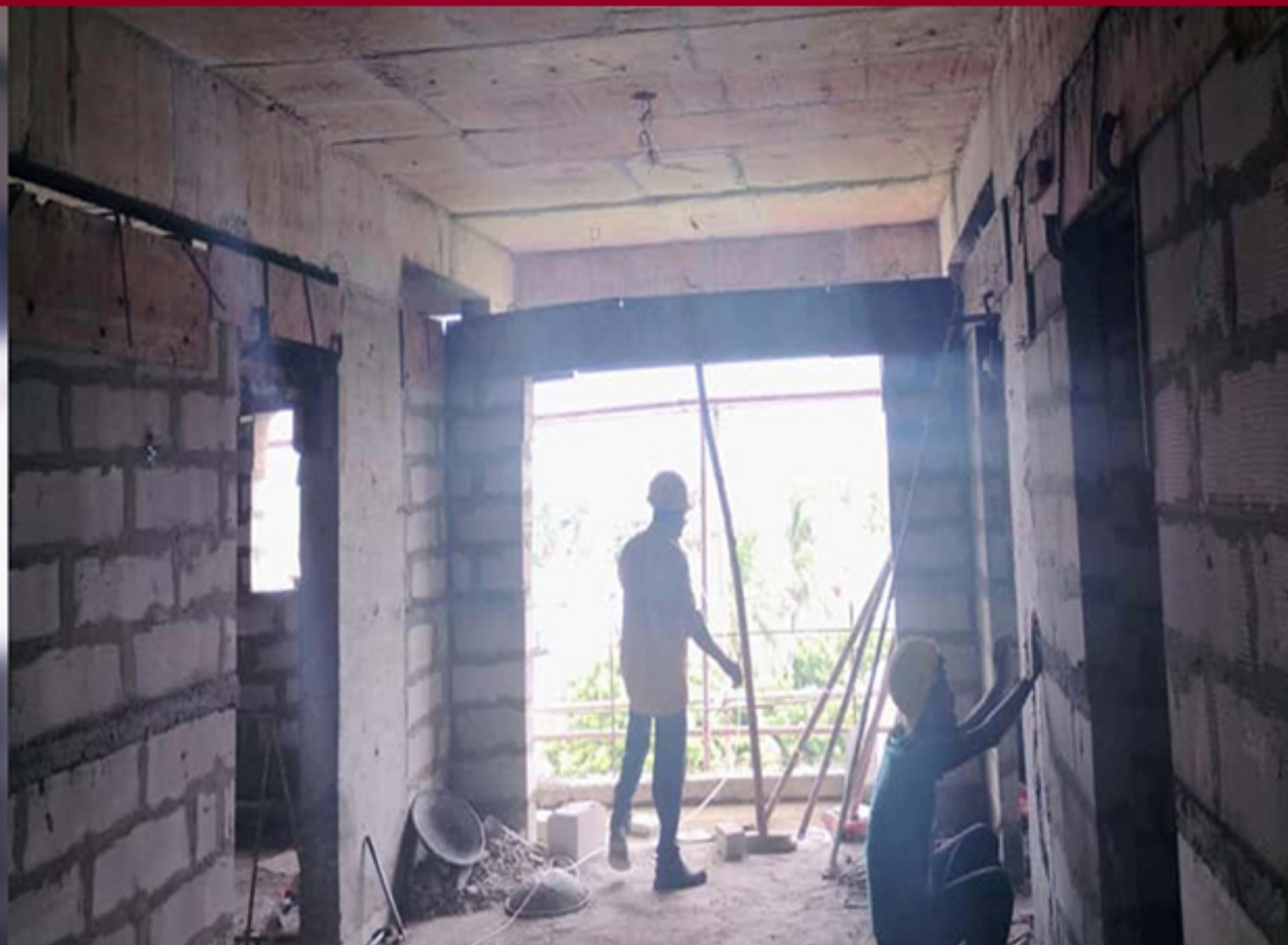
BLOCK 1 –CLUSTER B 5TH FLOOR LINTEL SHUTTERING WORK IN PROGRESS
